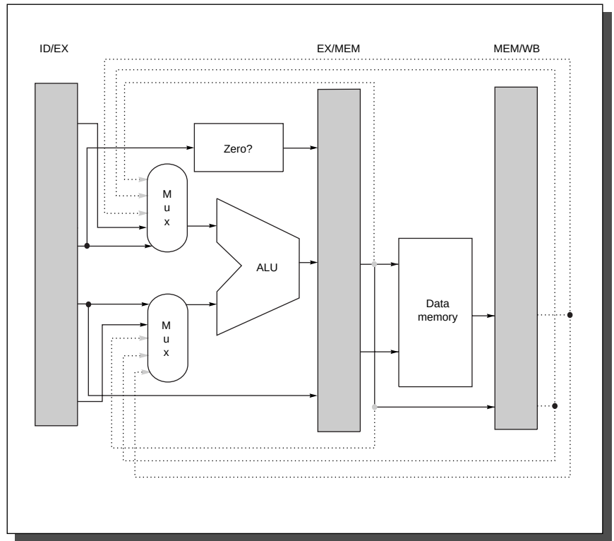
FIGURE 3.20 Forwarding of results to the ALU requires the addition of three extra inputs on each ALU multiplexer and the addition of three paths to the new inputs. The paths correspond to a bypass of (1) the ALU output at the end of the EX, (2) the ALU output at the end of the MEM stage, and (3) the memory output at the end of the MEM stage.
